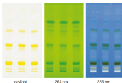
The chromatograms show as main compound naphthal yellow S. Other colored zones may appear.
